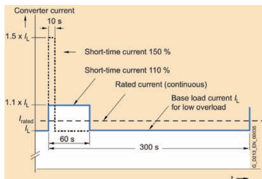
Load duty cycle definition for low overload
