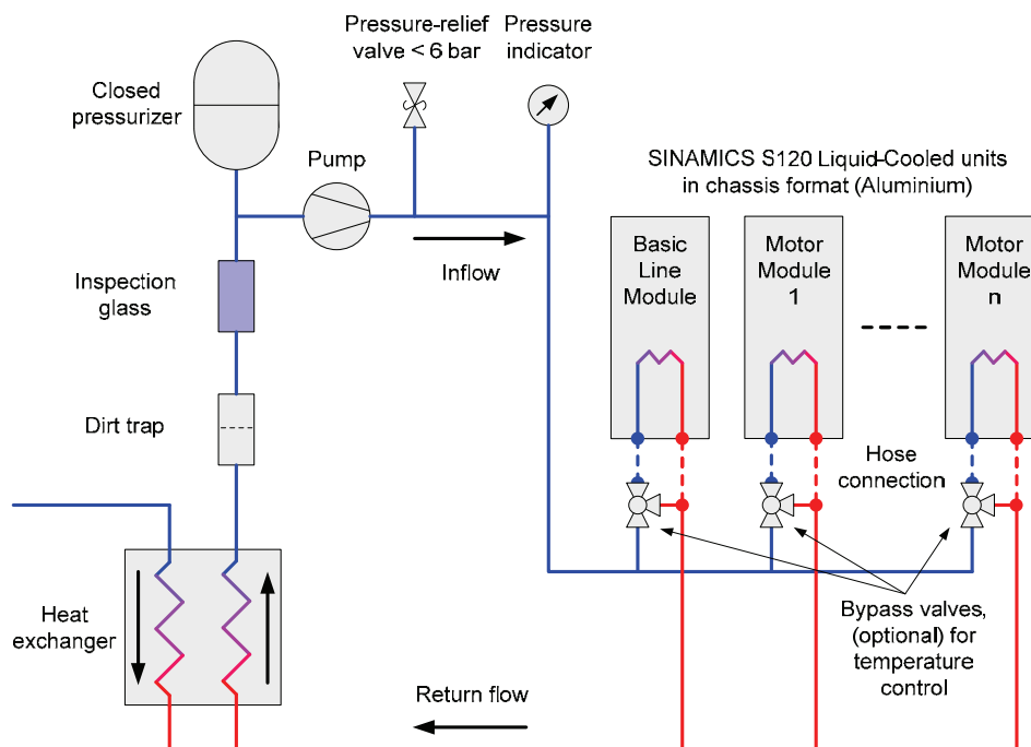
SINAMICS S120 Liquid-Cooled units in Chassis format: Recommendation for a closed cooling circuit
