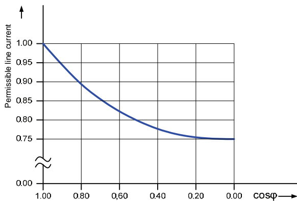
Permissible line current of the SINAMICS Active Infeed as a function of the line-side power factor \cos\phi
