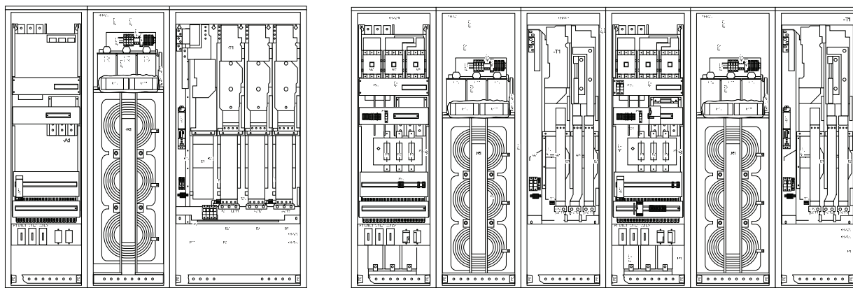
Examples of SINAMICS G150 and SINAMICS G150 parallel connections with integrated Line Harmonic Filter LHF compact
