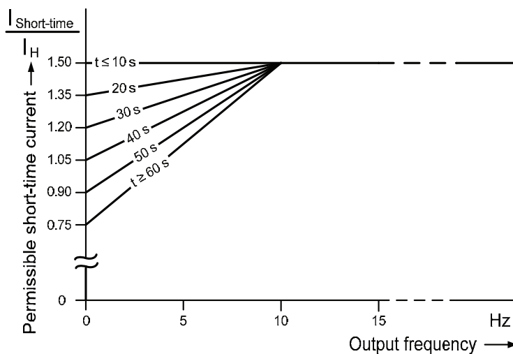
Permissible short-time current with occasional periods of high overload as a function of the output frequency and the overload period
