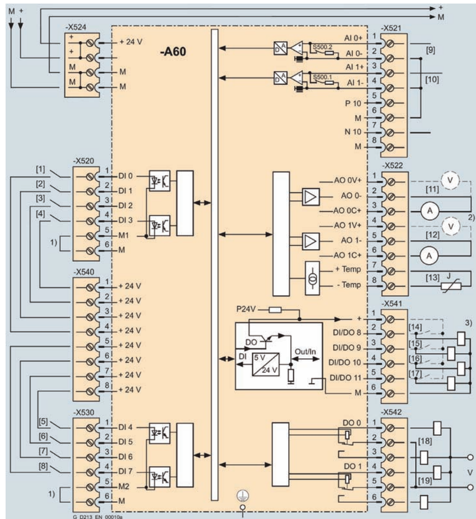
Optional customer terminal block on the TM31 Terminal Module (option G60)
