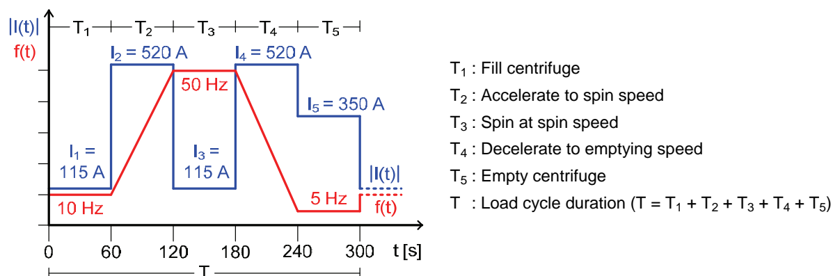
Absolute value of motor current |I(t)| and motor frequency f(t)
