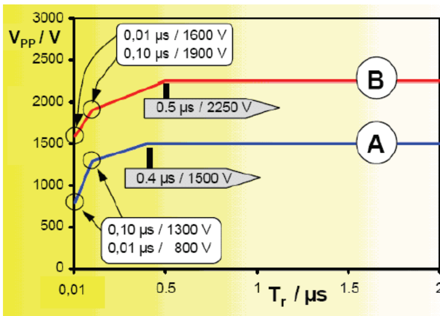
Permissible voltage limits \hat{U}_{PP} for trans-standard motors in the Siemens N-compact range:
