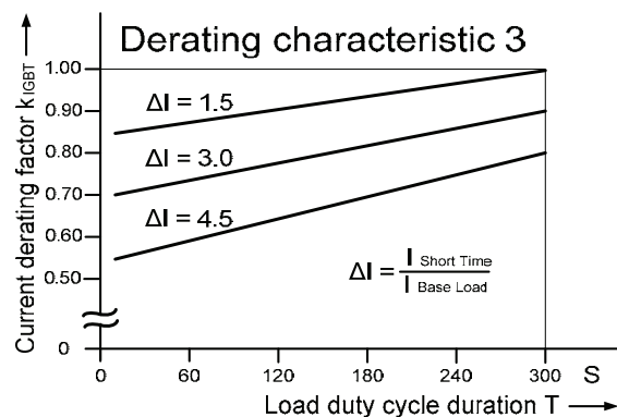
Derating factor k_{IGBT} as a function of the current ratio \Delta I = I_{ShortTime} / I_{BaseLoad} and the load duty cycle duration T
