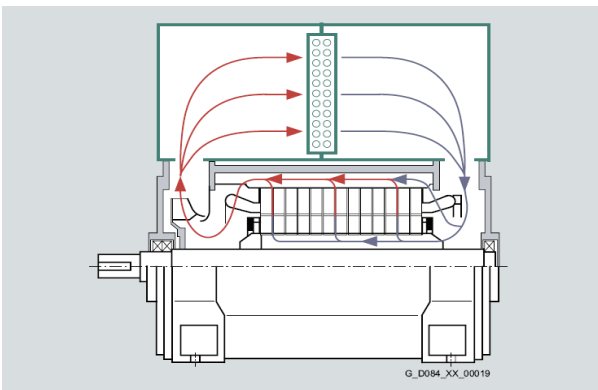
2a) Air/water heat exchange system / ventilation at one end
