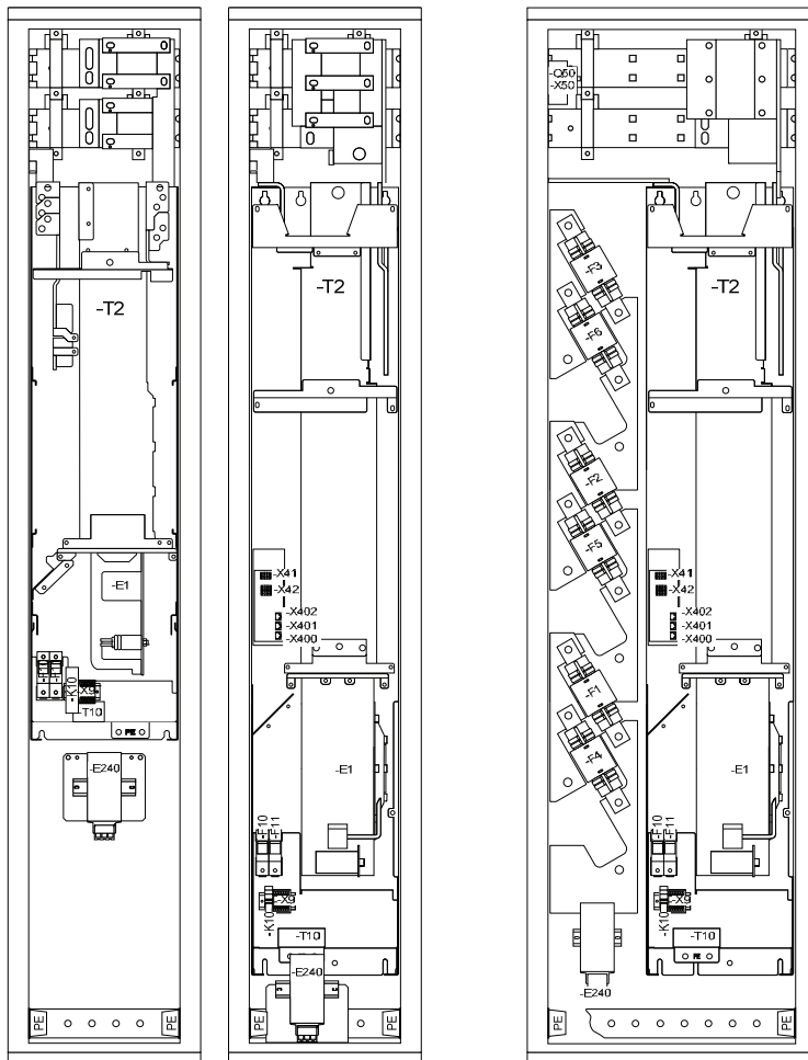
Basic Line Modules in frame sizes FB and GB / GD, and Basic Line Module for parallel connections
