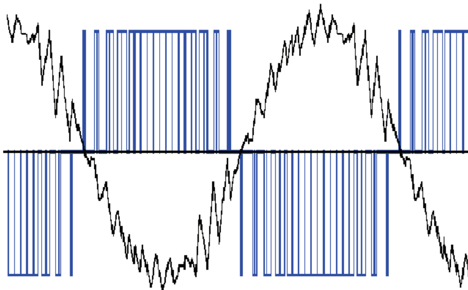
Motor voltage (phase-to-phase) and motor current with space vector modulation
