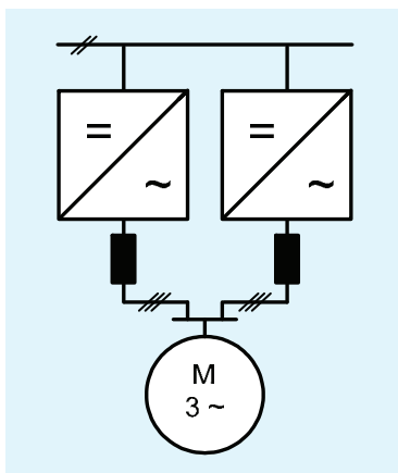
Use of motor reactors or filters if the cabling cannot be realized with the minimum required cable length
