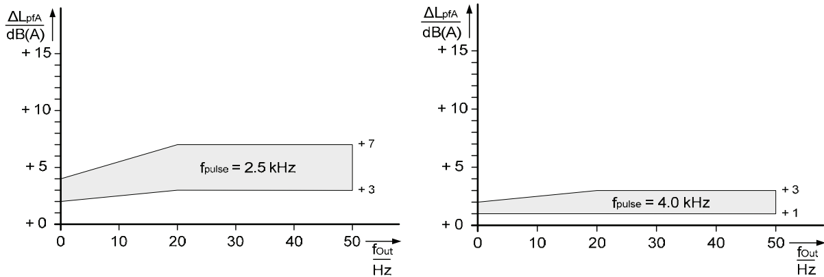
Increase in motor noise at pulse frequencies of 2.5 kHz or 4.0 kHz (i.e. at higher than factory-set pulse frequencies)
