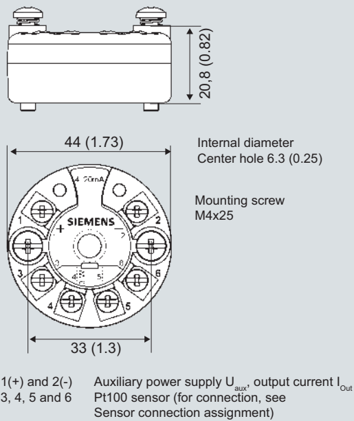
SITRANS TH100, dimensions in mm (inch)
