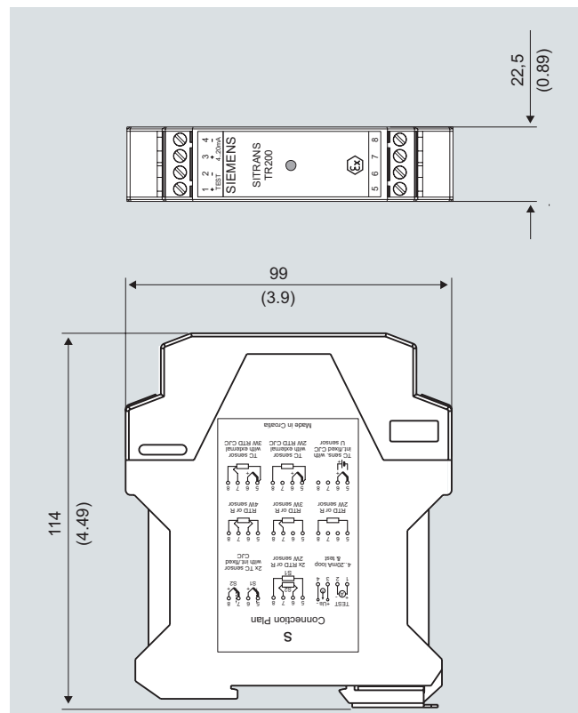
SITRANS TR200, dimensions in mm (inch)
