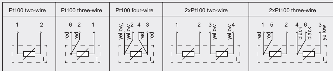
Connection diagram
