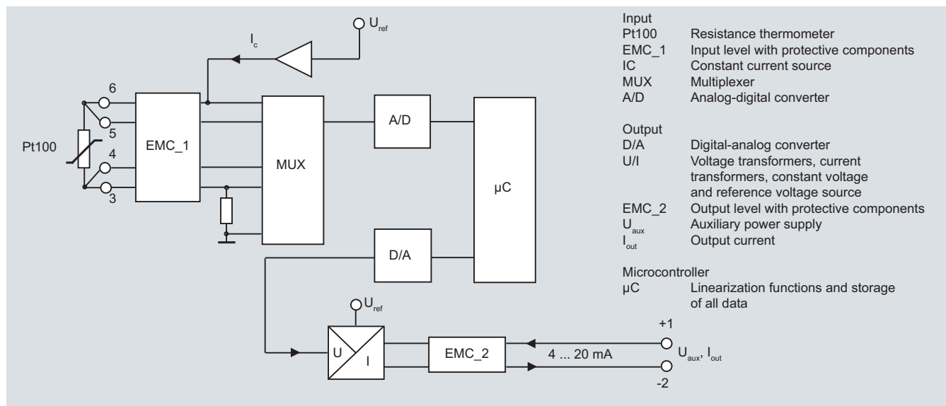
SITRANS TH100, function diagram
