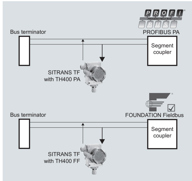
SITRANS TF with TH400, communication interface
