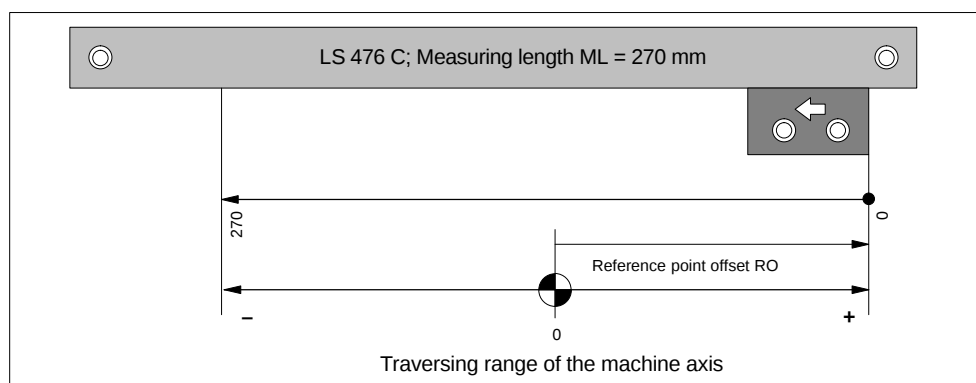
Fig. 4-3 Machine axis with linear encoder: Counterdirectional orientation
