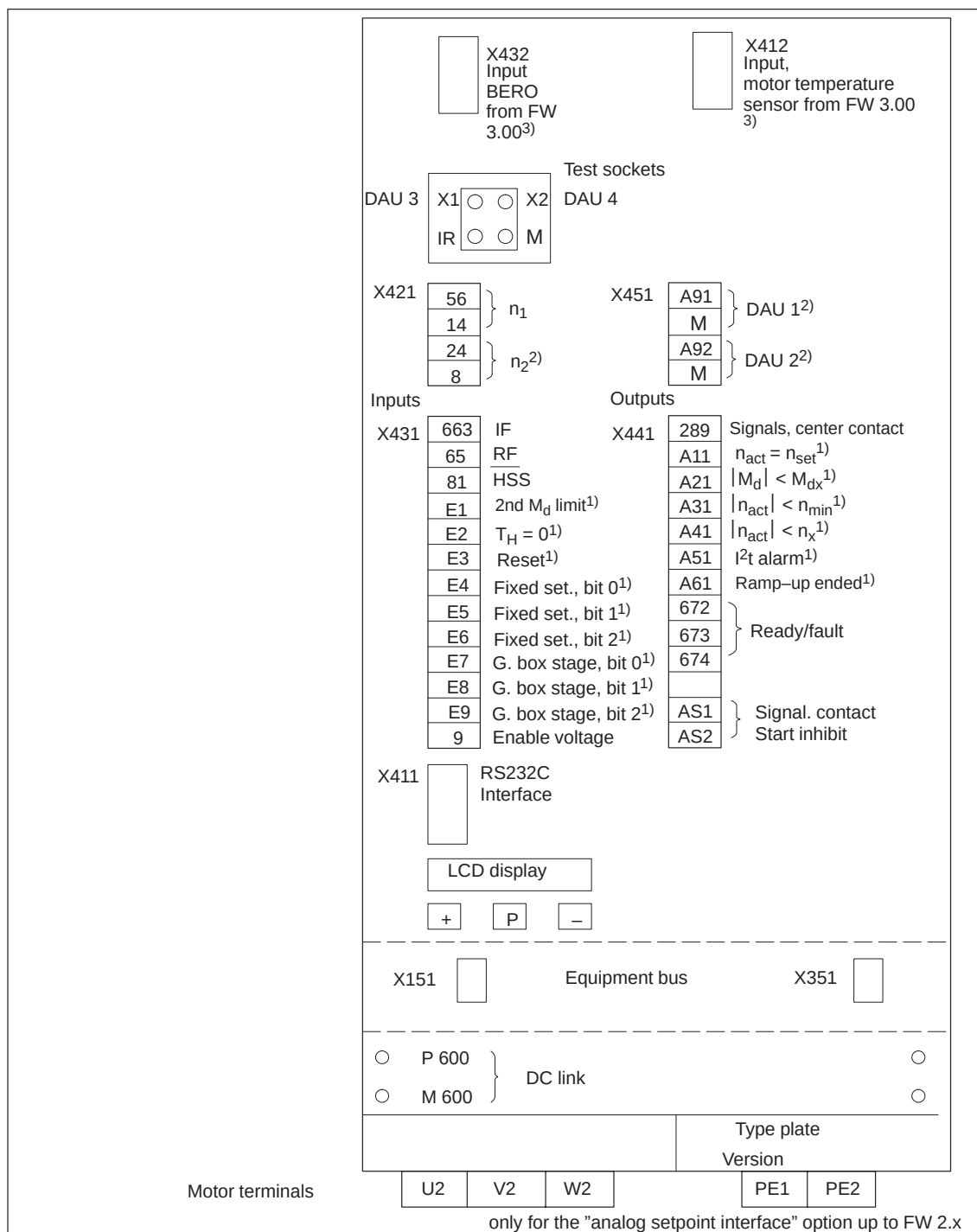
Fig. 1-3 Connections
