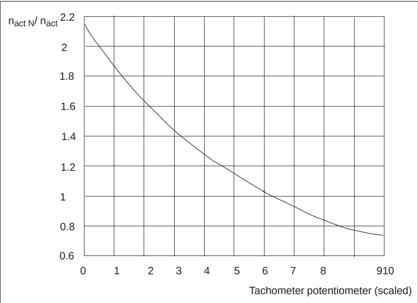
Fig. 2-1 Tachometer adjustment
