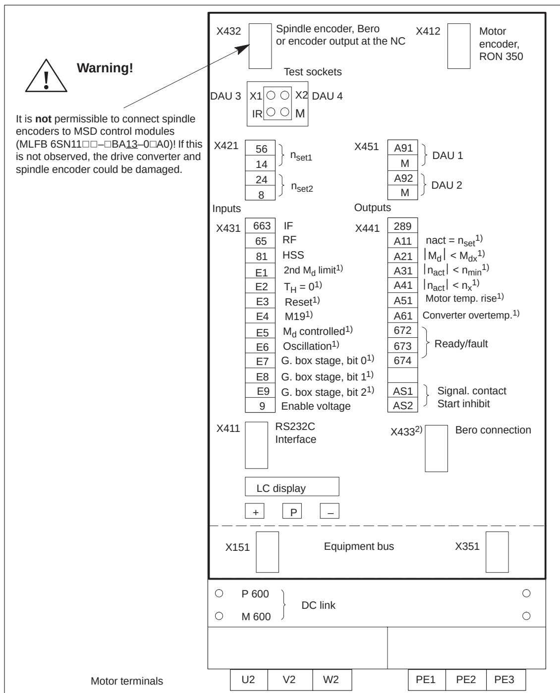
Fig. 1-3 Connections
