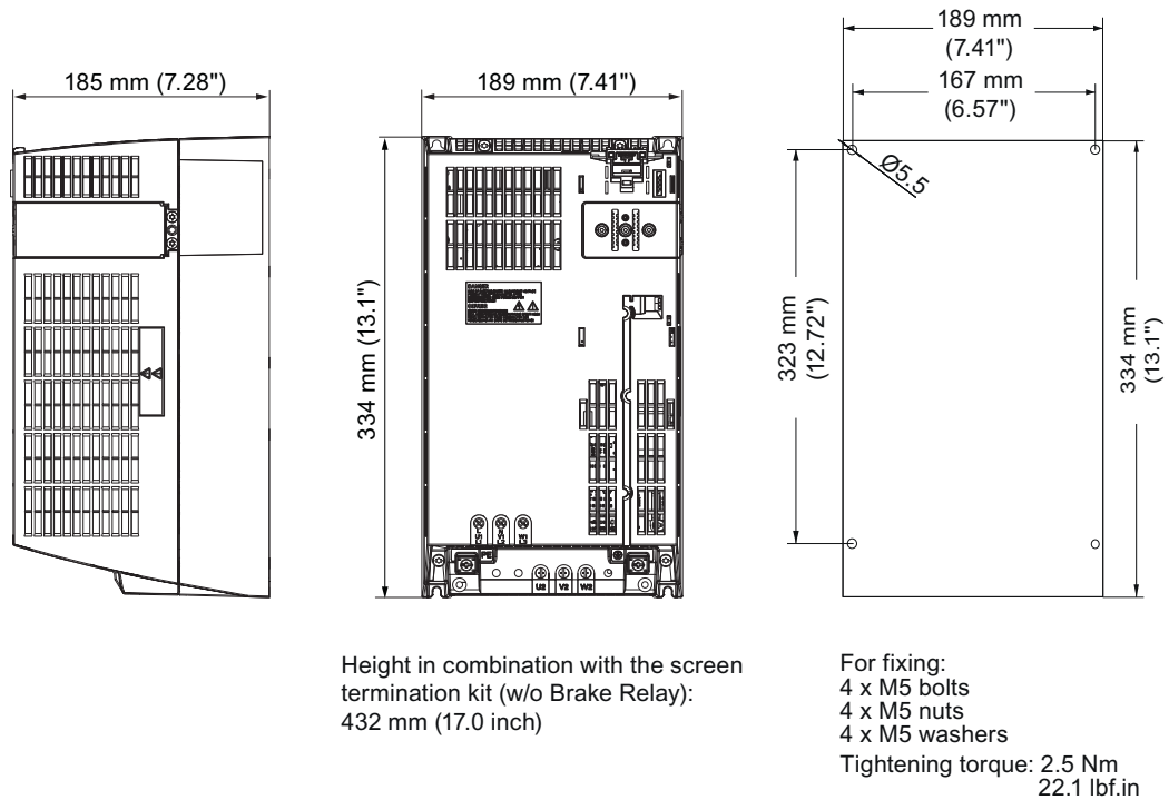
Figure 3-4 Dimensions and drill pattern for Power Module PM240, FSC, IP20
