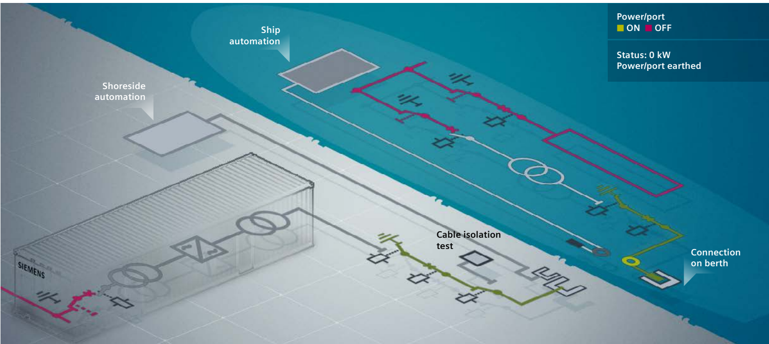
SIPLINK converter system for network applications in a SIHARBOR solution
