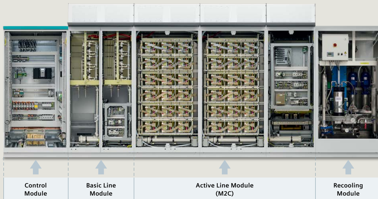
Medium-voltage converter SINAMICS SM120 CM (cabinet modules)
